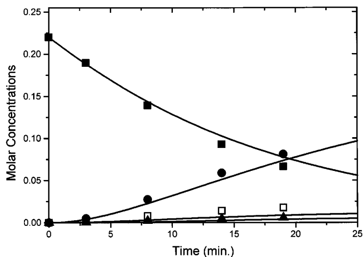
Figure 3. Reaction of benzaldehyde with lithium in THF at 48 °C. Experimental data: ■, benzaldehyde; ●, benzyl alcohol; ▲, benzil; □, benzoin. Simulated curves
