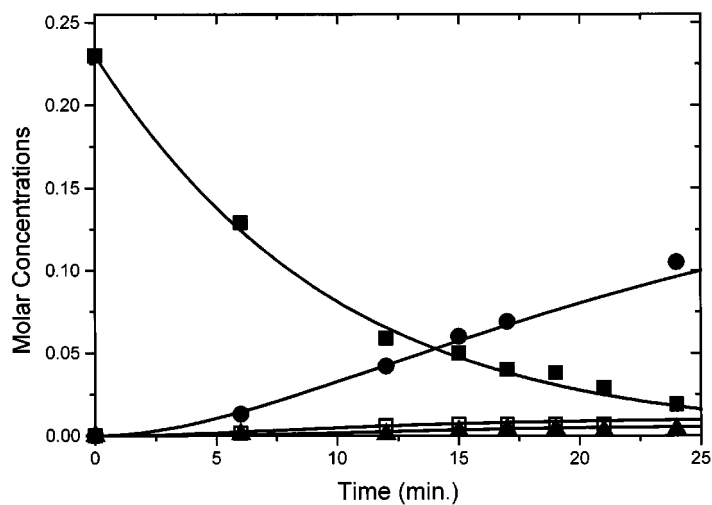
Figure 4. Reaction of benzaldehyde with lithium in THF at 58 °C. Experimental data: ■, benzaldehyde; ●, benzyl alcohol; ▲, benzil; □, benzoin. Simulated curves
