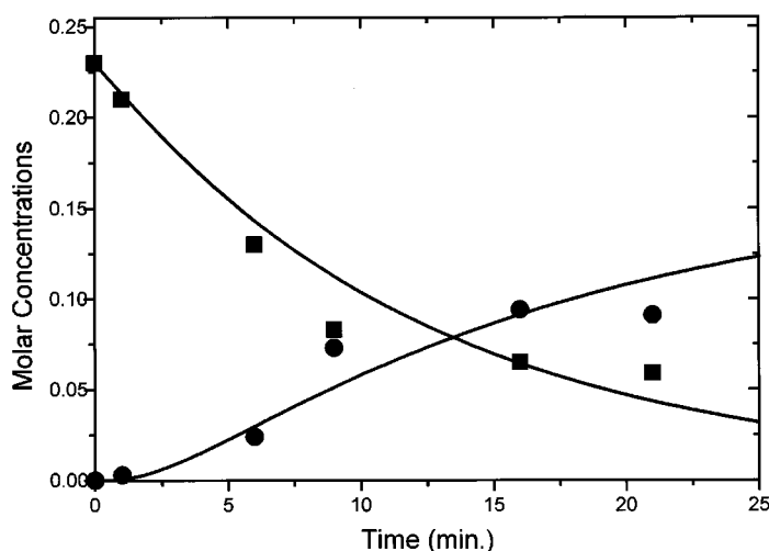
Figure 2. Reaction of benzaldehyde with lithium in THF at 37 °C. Experimental data: ■, benzaldehyde; ●, benzyl alcohol. Simulated curves
