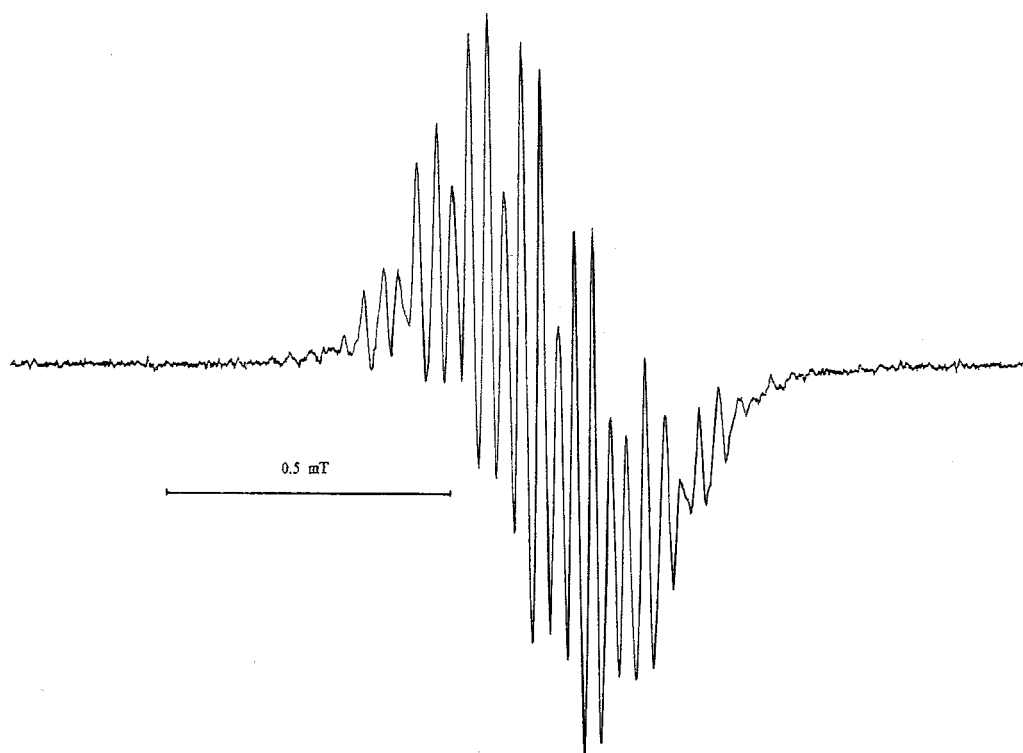
Figure 1. EPR spectrum of the reaction mixture of benzaldehyde with lithium metal in THF. Modulation amplitude 10 = 1.6 gain 10^{-5} = 4 ; spectral width \Delta = 0.9 mT (coincident with the EPR spectrum of benzil radical anion under the same conditions)
